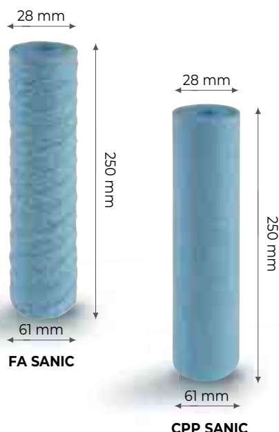
CPP SANIC
